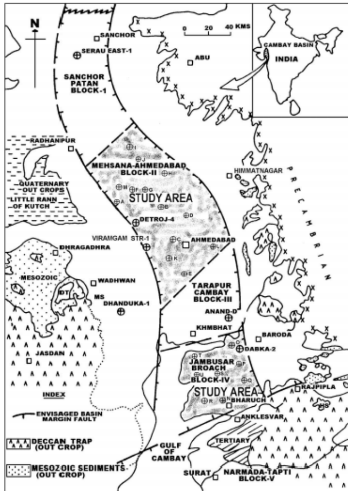
Figure XII-2. Cambay Basin Study Area.
