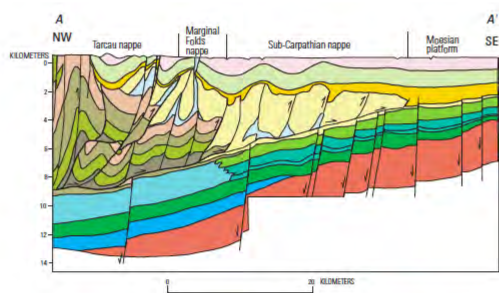
Figure VI-17. Carpathian-Balknian Basin Cross Section
