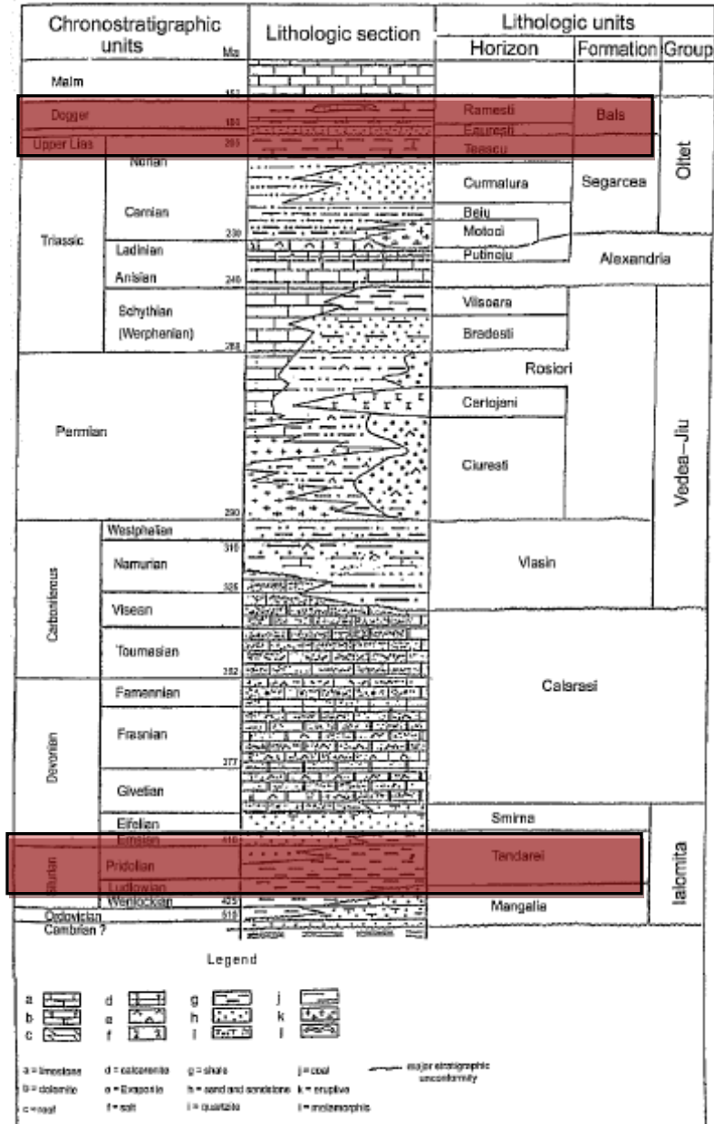
Figure VI-15. Carpathian-Balkanian Stratigraphic Column
