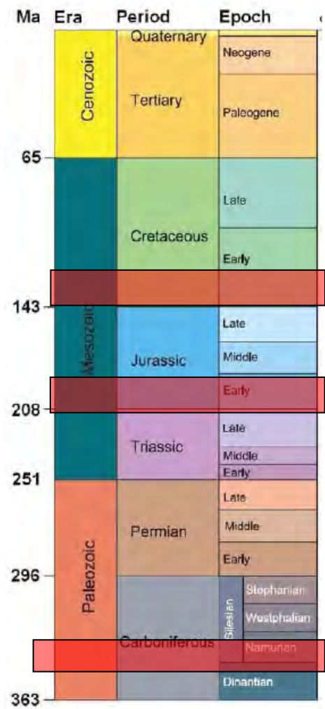
Figure VII-11. North Sea-German Basin Stratigraphic Column9
