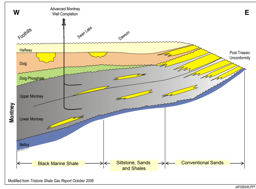
Figure I-11. Montney and Doig Resource Plays, Stratigraphy
