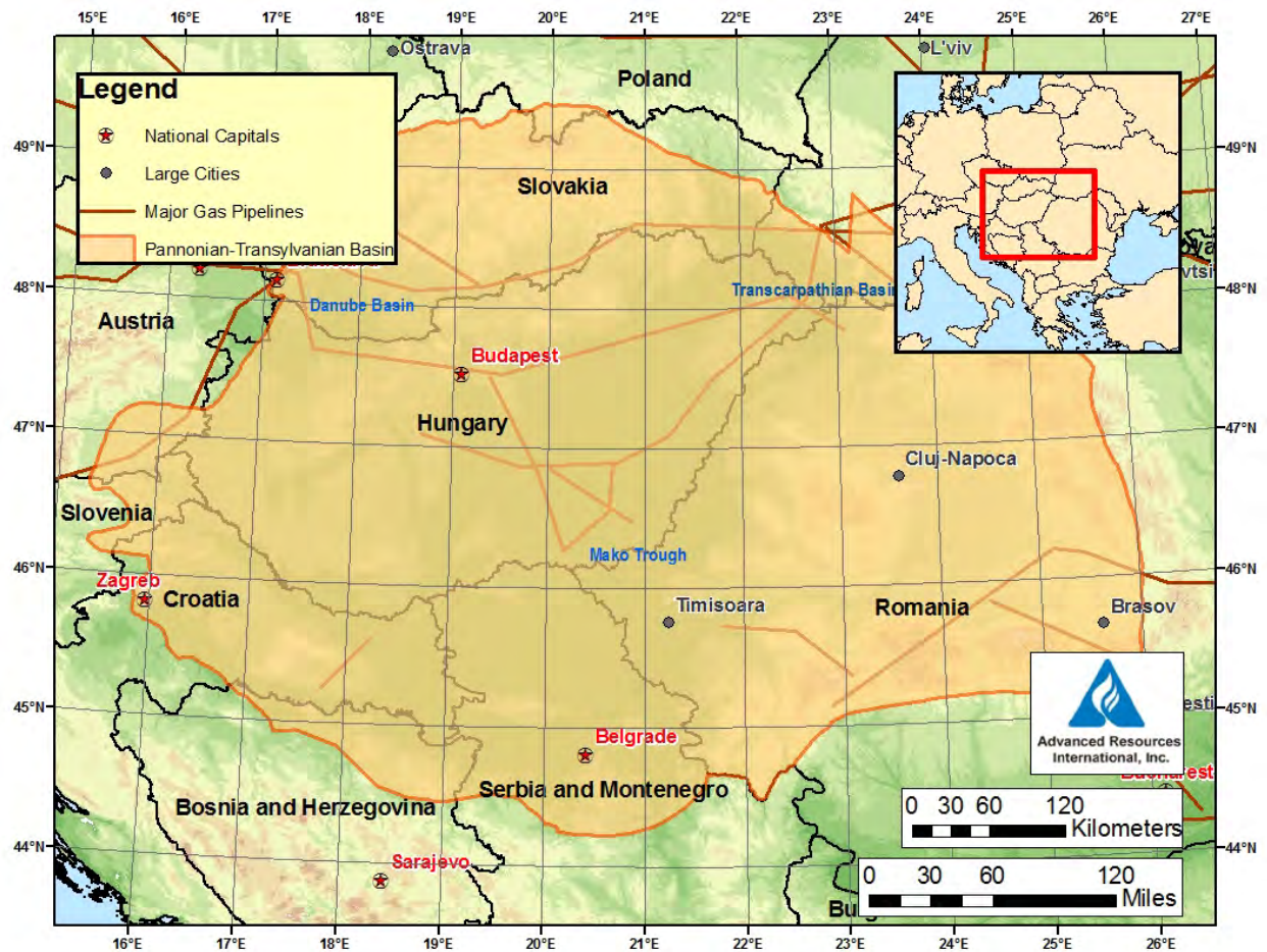
Figure VI-11. Pannonian-Transylvanian Basin
